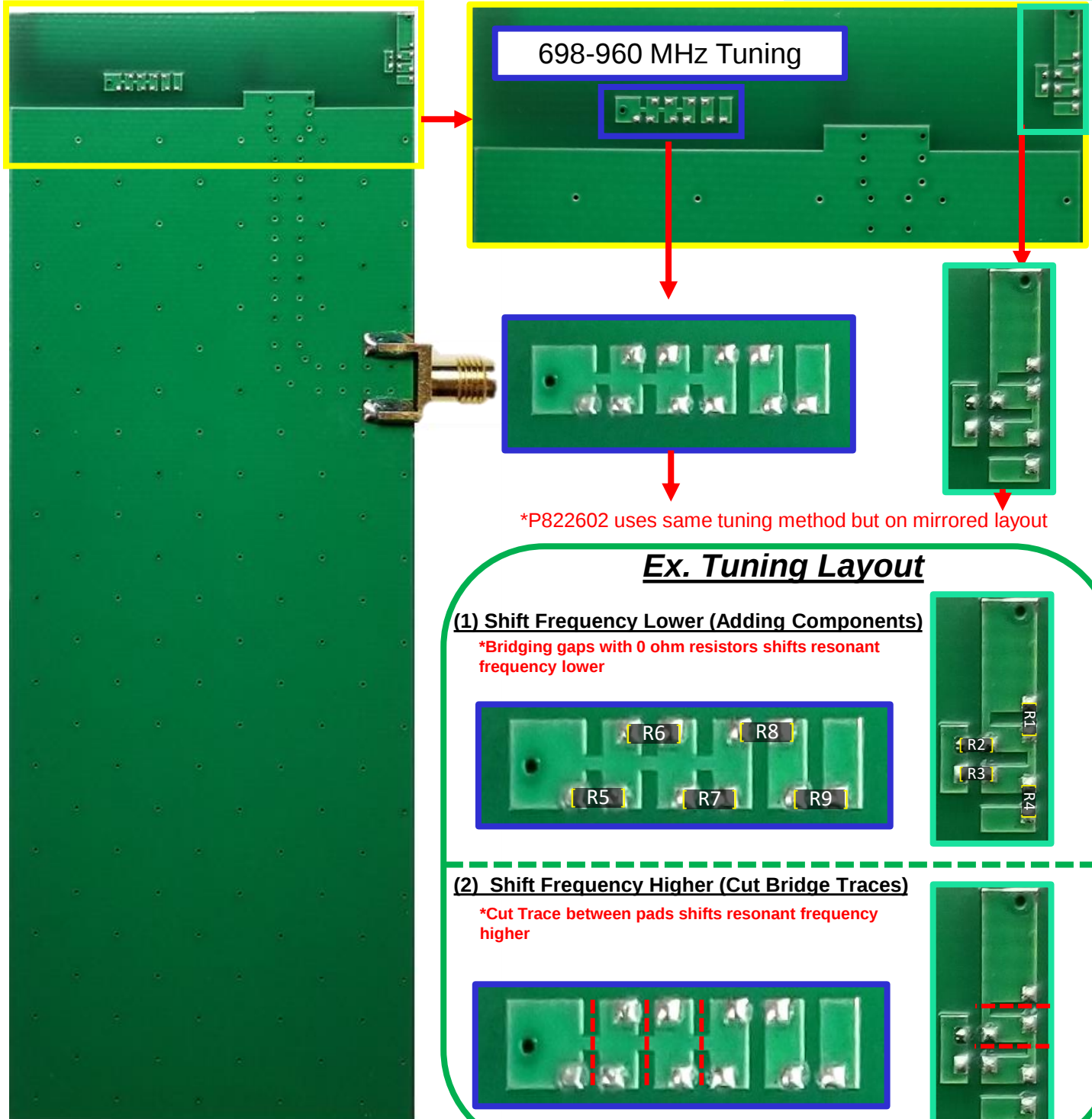
Demo Board Back
