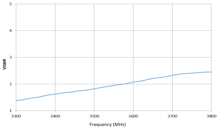
n78 VSWR
