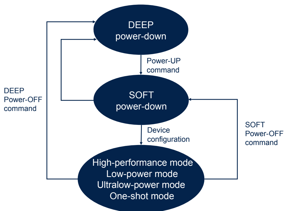
Figure 8. Power-up sequence
